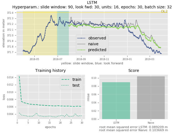
Fig. 16. Long-term forecast with k = 90 and n = 30 on one-year data
