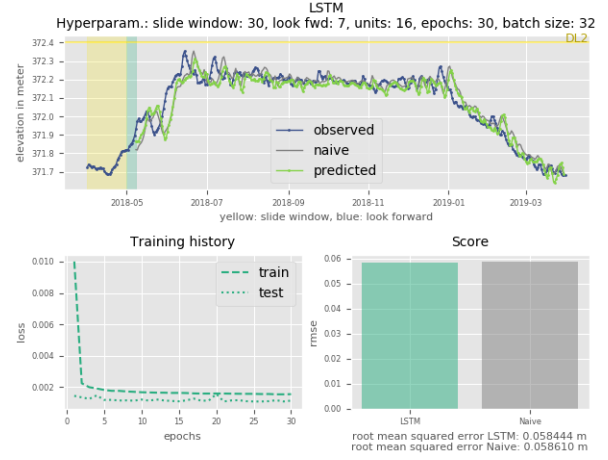
Fig. 15. Medium-term forecast with k = 30 and n = 7 on one-year data
