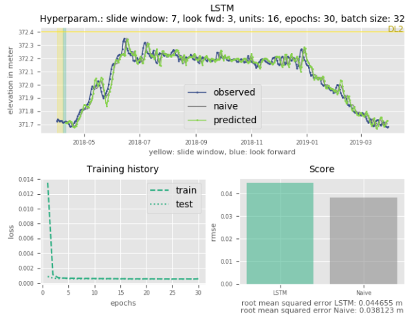
Fig. 14. Short-term forecast with k = 7 and n = 3 on one-year data
