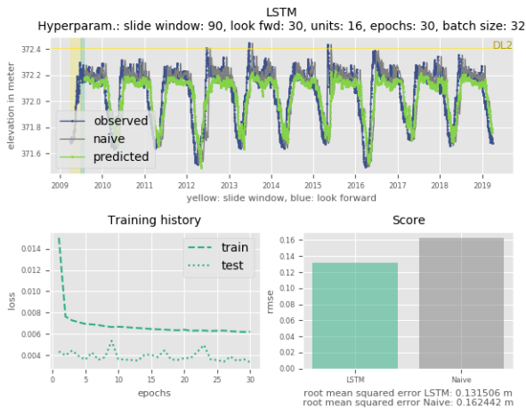
Fig. 17. Long-term forecast with k = 90 and n = 30 on ten-years data
